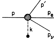
FIG. 12. The induced \beta decay in the presence of the pion condensate.
