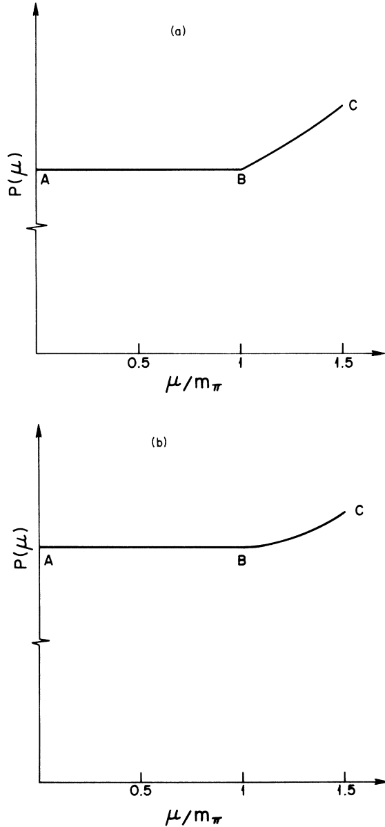
FIG. 2. The pressure vs the chemical potential. (a) In the (m_\pi^2/2)\pi^2 symmetry breaking. For AB, P(\mu) = (\lambda^2/4)f_\pi^4 ; the pressure is independent of \mu . For BC, P(\mu) = (\lambda^2/4)[f_\pi^2 + (\mu^2 - m_\pi^2)/\lambda^2] . Notice the discontinuity in dP/d\mu at \mu = m_\pi . (b) In the f_\pi m_\pi^2 \sigma symmetry breaking. For AB, P(\mu) = (\lambda^2/4)f_\pi^4 + (m_\pi^2 f_\pi^2/2) . For BC, P(\mu) = (\lambda^2/4)[f_\pi^2 + (\mu^2 - m_\pi^2)/\lambda^2] + (f_\pi^2 m_\pi^4/2\mu^2) . At \mu = m_\pi , P(\mu) and dP/d\mu are continuous but d^2P/d\mu^2 is not.
