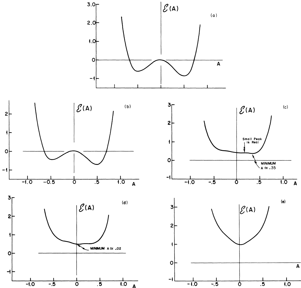
FIG. 13. The ground-state energy-density function \mathcal{E}_0(\rho_B, A) plotted vs A . (a) p_F = 0, \rho_B = 0 , (b) p_F = 1, \rho_B = 0.2\rho_B^{\text{nucl}} , (c) p_F = 2, \rho_B = 1.59\rho_B^{\text{nucl}} , (d) p_F = 2.1, \rho_B = 1.84\rho_B^{\text{nucl}} , (e) p_F = 2.5, \rho_B = 3.10\rho_B^{\text{nucl}} .
